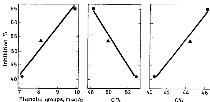
FIG. 2. Correlations between phenolic groups, oxygen and carbon contents of different soil fulvic acids at 40 mg/l and their IAA oxidation inhibition. (●) meadow; (▲) forest; (■) cultivated soils.
